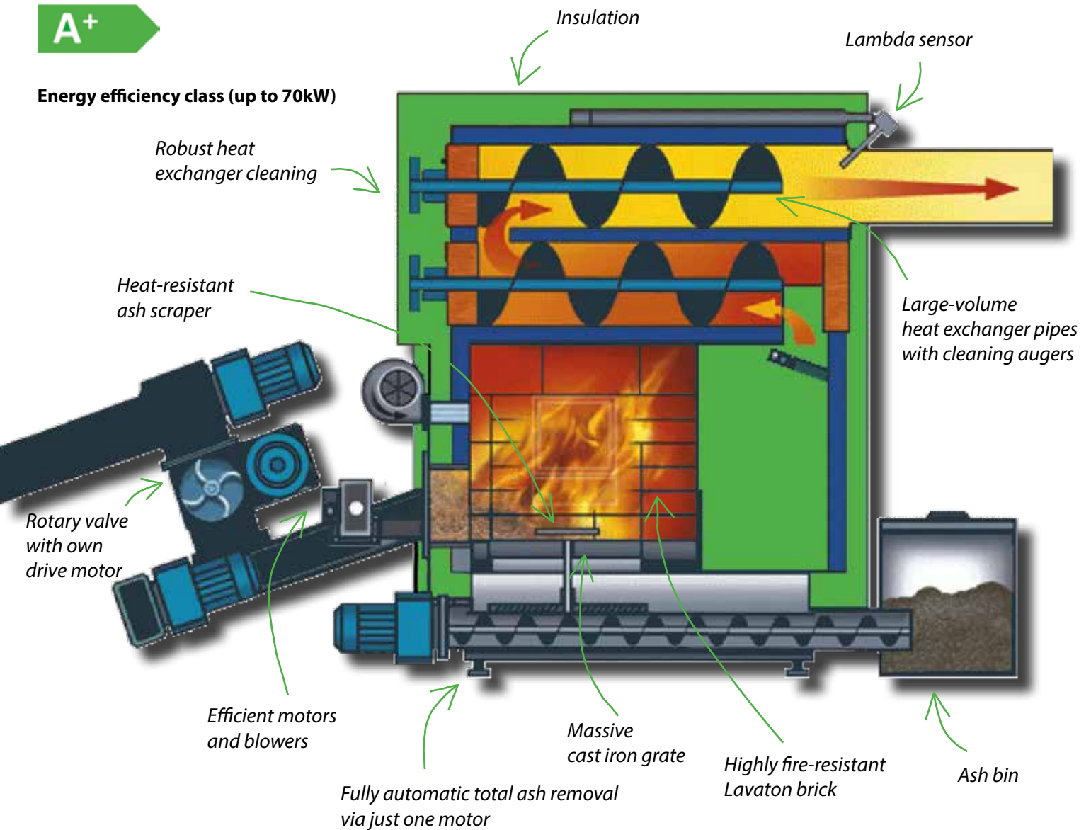
HSK-RA 60 built in 2007
